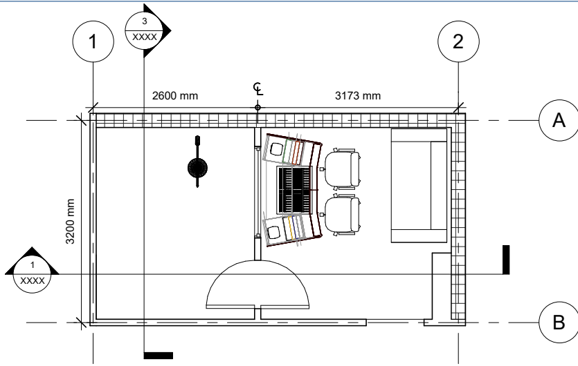
2 Plan View 1 : 50
